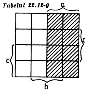
Fig. 22.12. a) — Numerotarea căsuțelor; b) — f(a, b, c, d) = abd ; c) — f(a, b, c, d) = bcd ; d) — f(a, b, c, d) = b \cdot c ; e) — f(a, b, c, d) = b \cdot c ; f) — f(a, b, c, d) = d ; g) — f(a, b, c, d) = a
