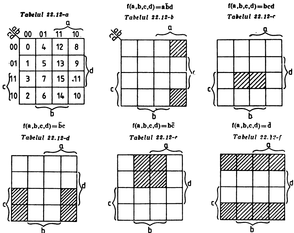
Fig. 22.12. a) — Numerotarea căsuțelor; b) — f(a, b, c, d) = abd ; c) — f(a, b, c, d) = bcd ; d) — f(a, b, c, d) = b \cdot c ; e) — f(a, b, c, d) = b \cdot c ; f) — f(a, b, c, d) = d ; g) — f(a, b, c, d) = a
